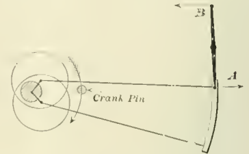
FIG. 10. REGULAR INDIRECT MOTION WITH ROCKER.
